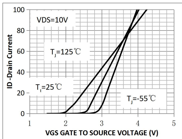
Figure 10. Transfer Characteristics
